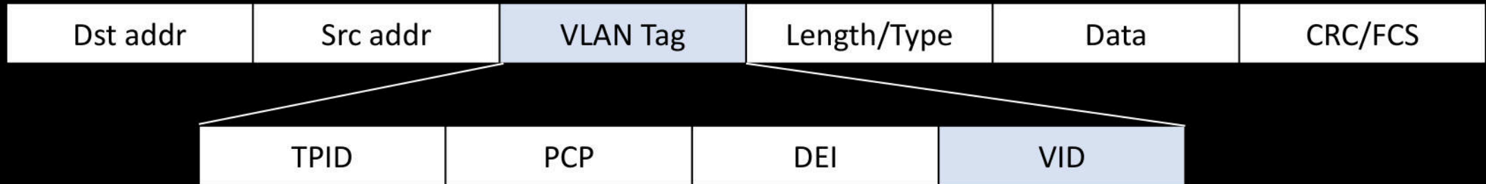
Ethernet frame with VLAN tag
